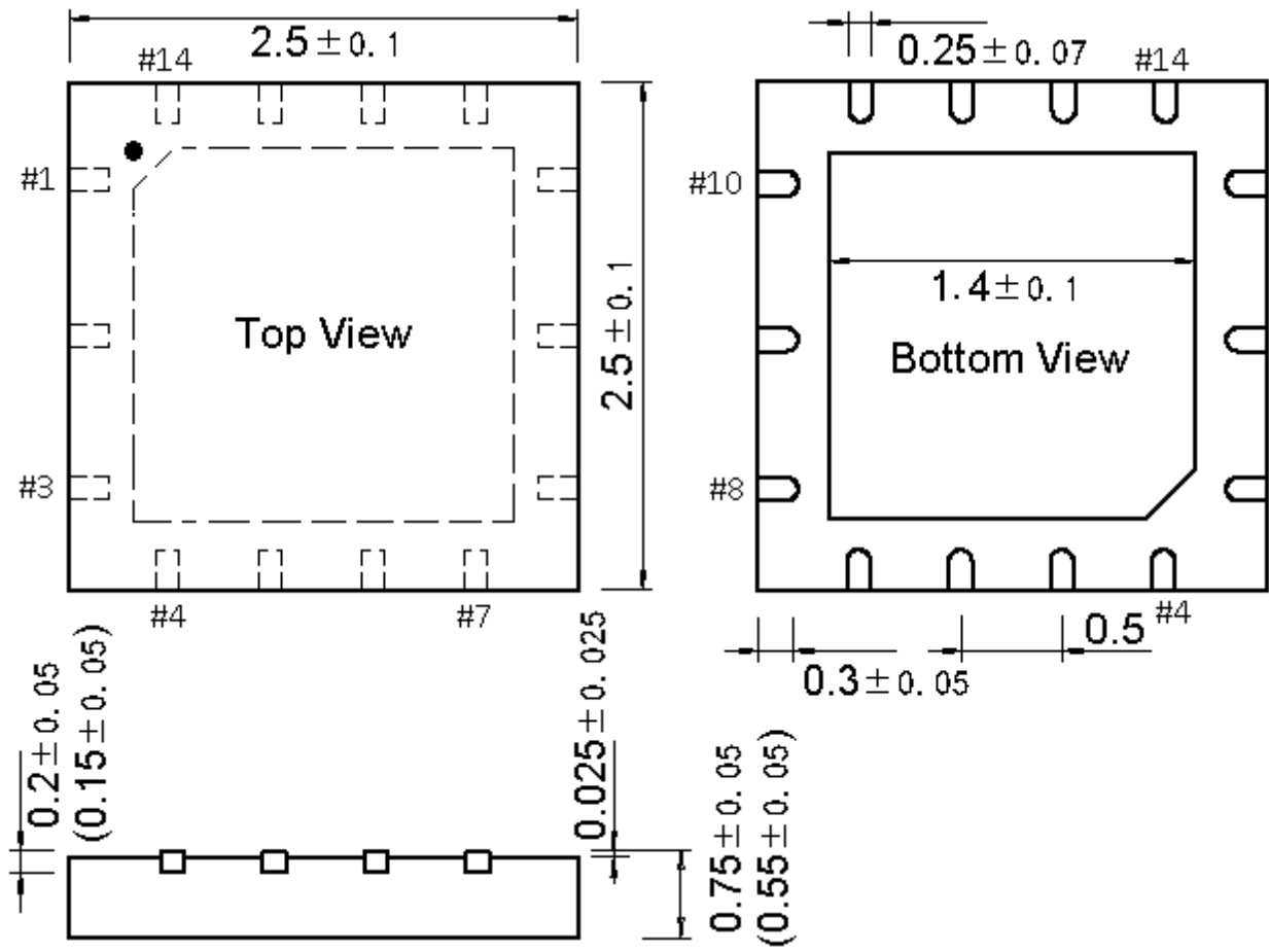
QFN14 (QFN14-2.5*2.5*0.75-0.5)
