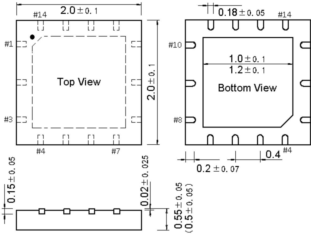
QFN14X2 (QFN14-2*2*0.55-0.4)
