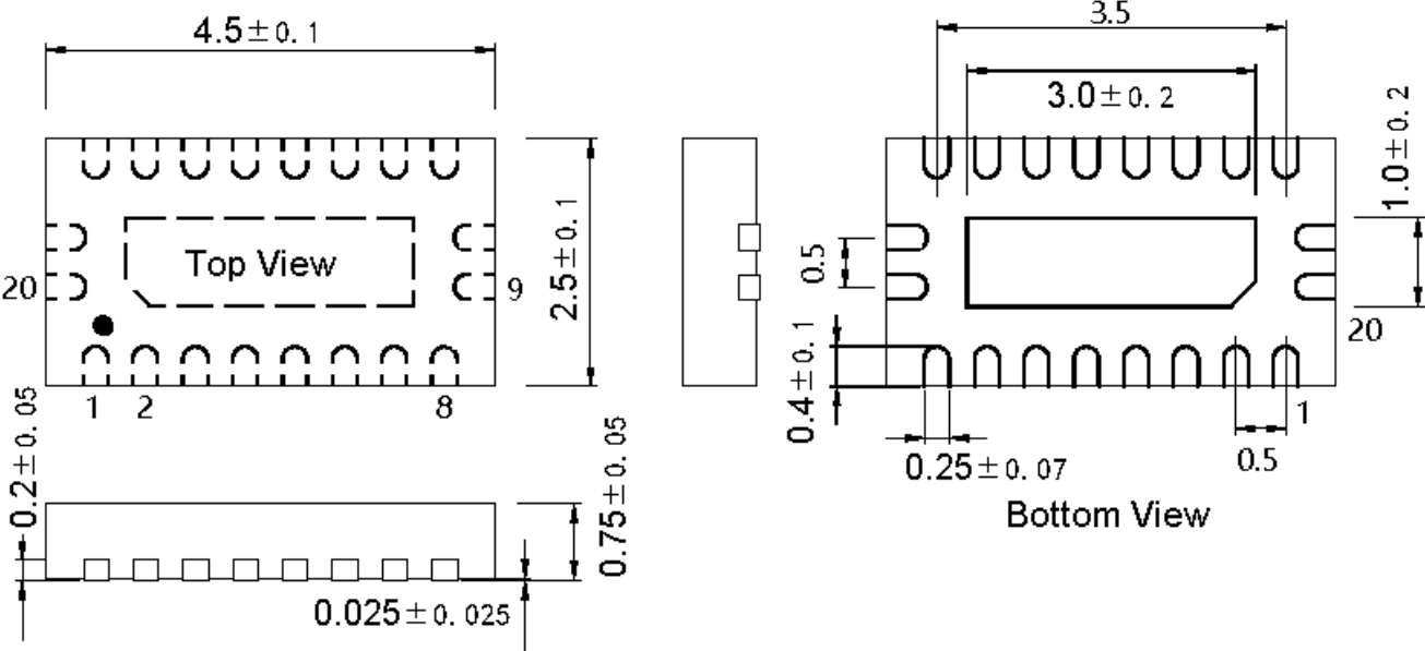
QFN20-2.5*4.5
