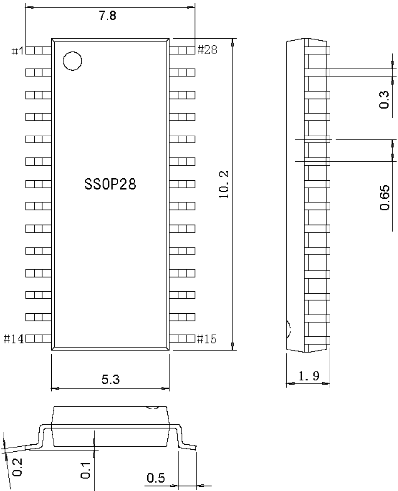
SSOP28 (SSOP28-209mil-0.65)
